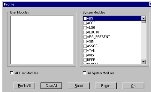
Figure 12-4: Profile Dialog
