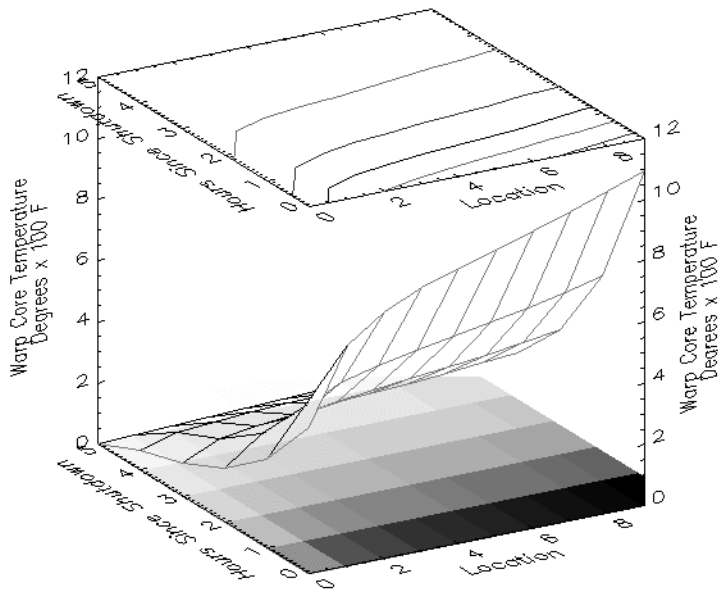
Figure 0-1: SHOW3 result of unlimited dimensions example
